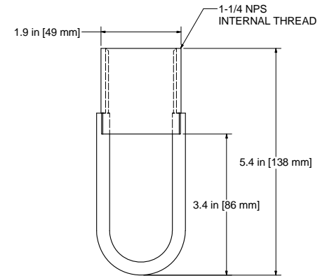
CT-400 MOUNTING BRACKET
