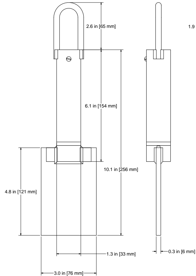
CT-200GC COMPACT PROBE WITH PADDLE
