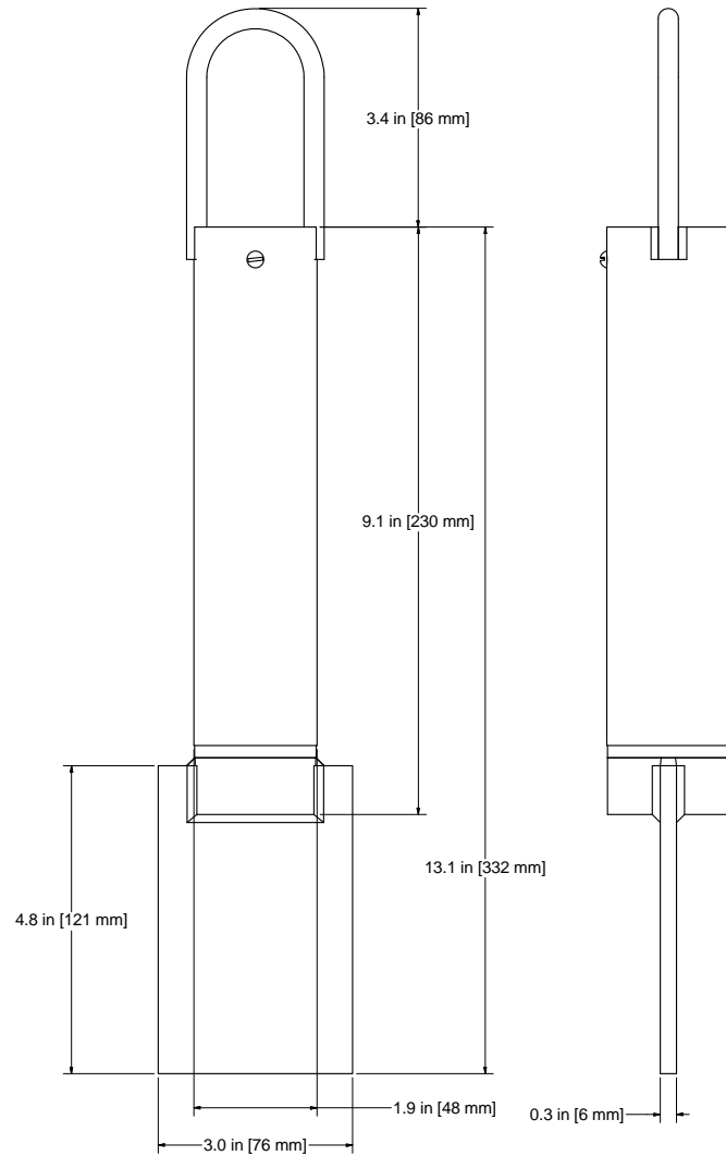
CT-201GP STANDARD SIZE PROBE WITH PADDLE
